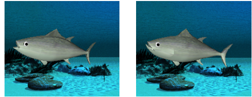
Figure 8: Fish animation.
