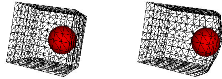
Figure 9: Bouncing sphere.
